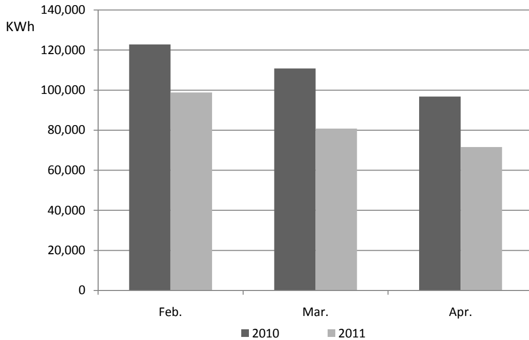
Fig. 5-4 Electricity Consumption Comparison before and after the Schedule and Mode Optimization Fan
